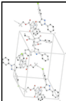
Fig. 3. A partial view of the crystal packing of the title compound. H atoms not involved in the C—H...O and C—H...Cl interactions (dashed lines) have been omitted for clarity.
